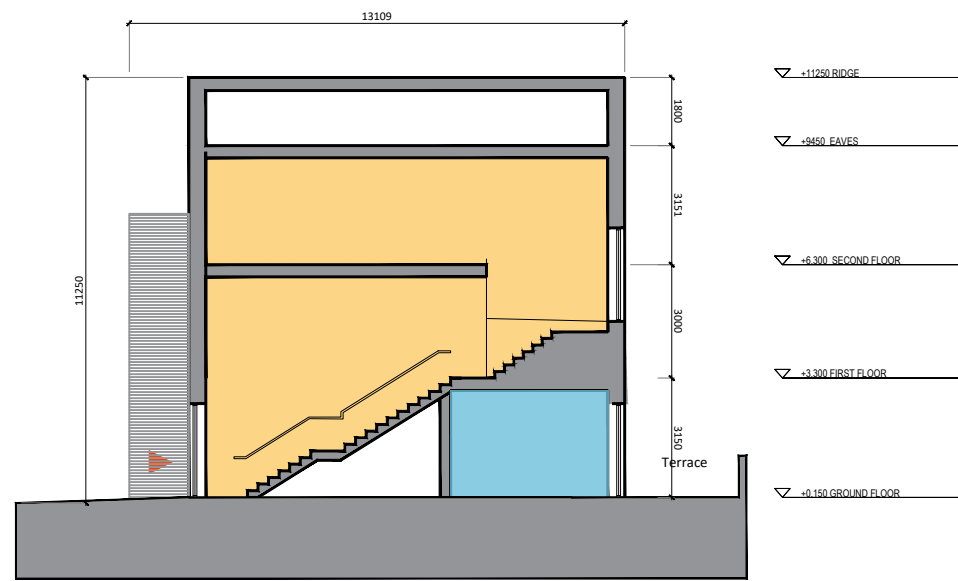
Section 1:200
